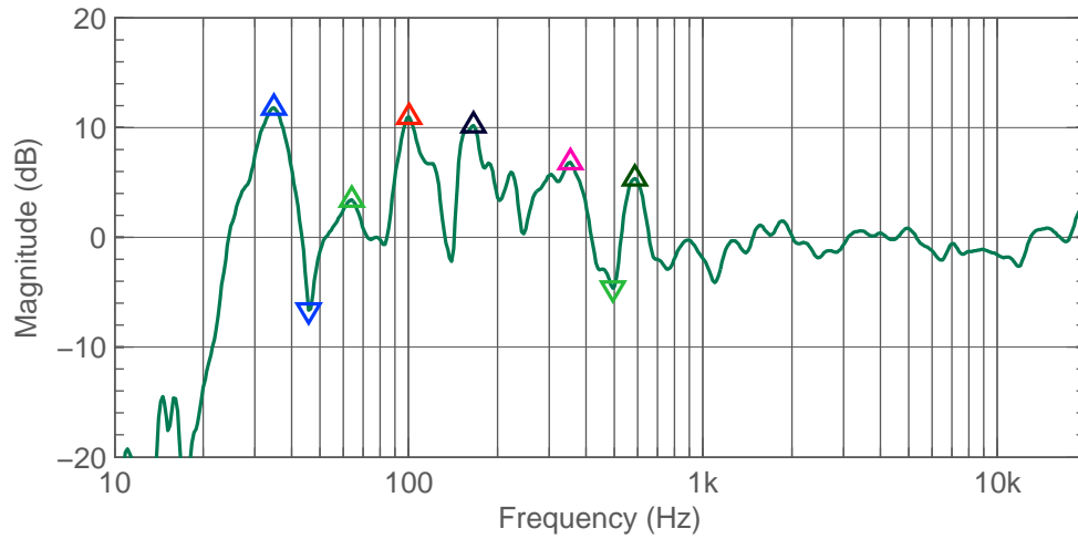
Figure 3.6: Left 8351B peaks and notches (before calibration).
