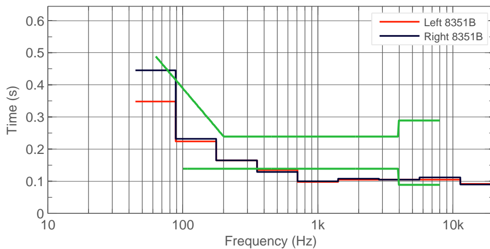
Figure 6.4: Decay time T60, after calibration. Target decay time T_m = 0.19 s (based on calculated room volume).
