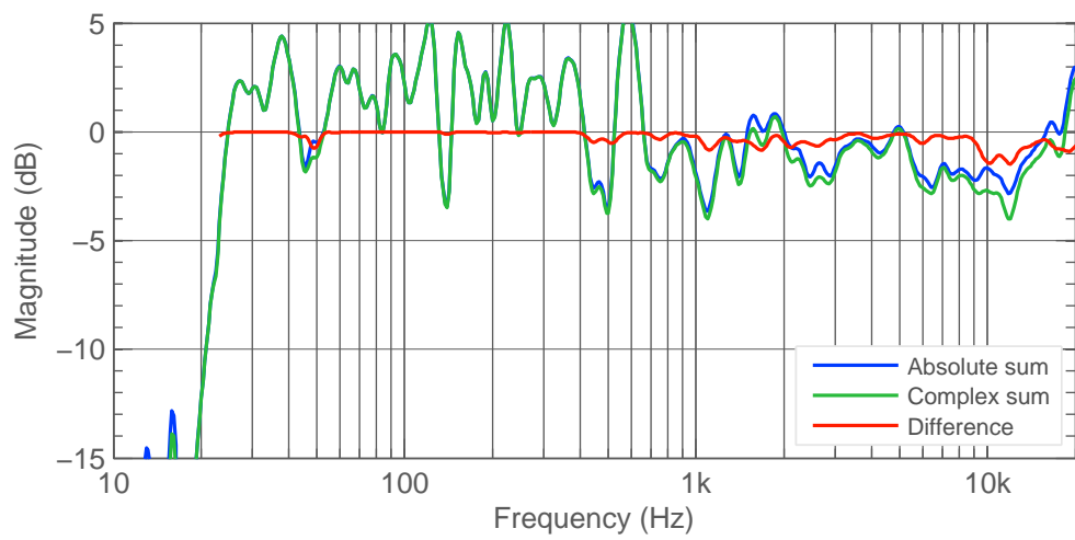
Figure 3.5: Difference between the sum of complex pressure and sum of absolute pressure. Calibration group ID 1.
