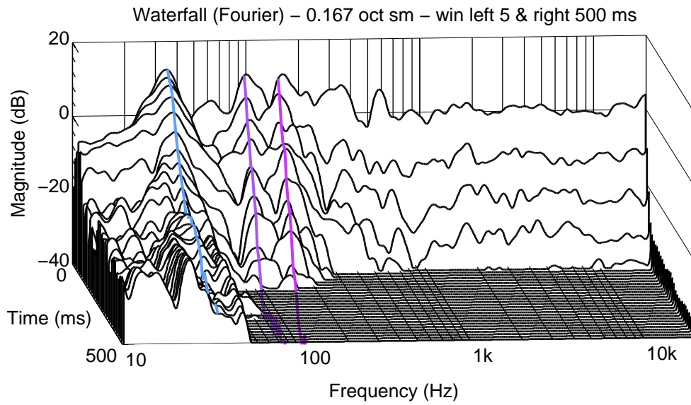
Figure 5.3: Left 8351B. Waterfall.
