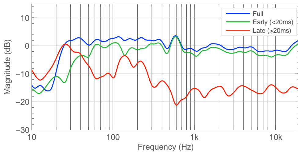
Figure 4.8: Right 8351B. Full, early and late frequency response.
