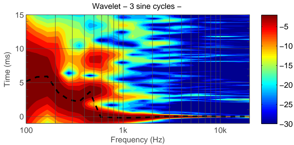
Figure 5.8: Left 8351B. Wavelet.
