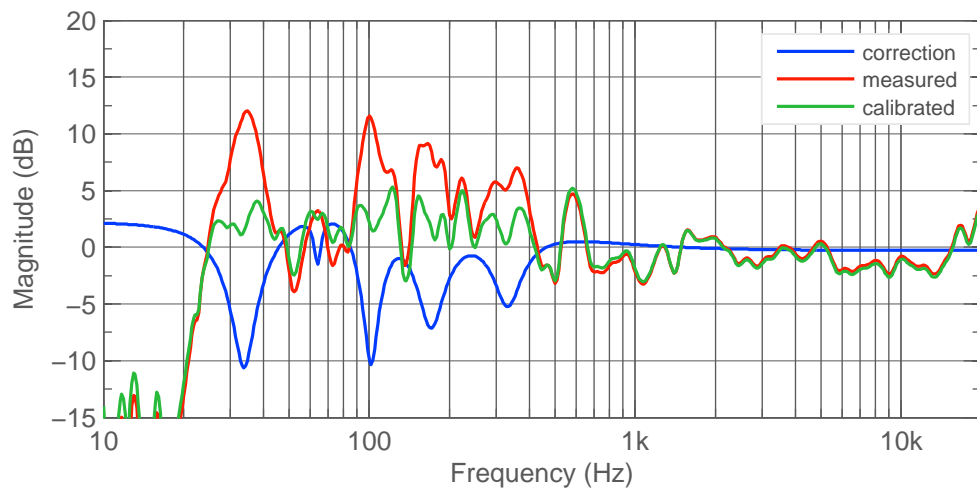
Figure 3.2: Right 8351B frequency response.
