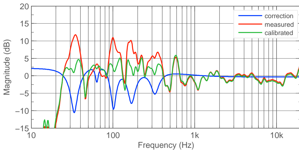
Figure 3.1: Left 8351B frequency response.
