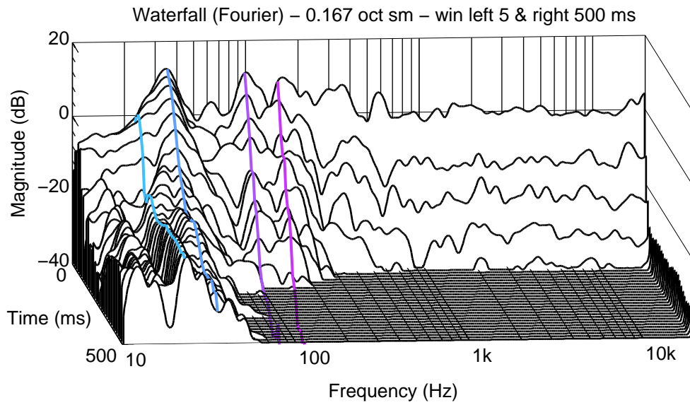
Figure 5.5: Right 8351B. Waterfall.
