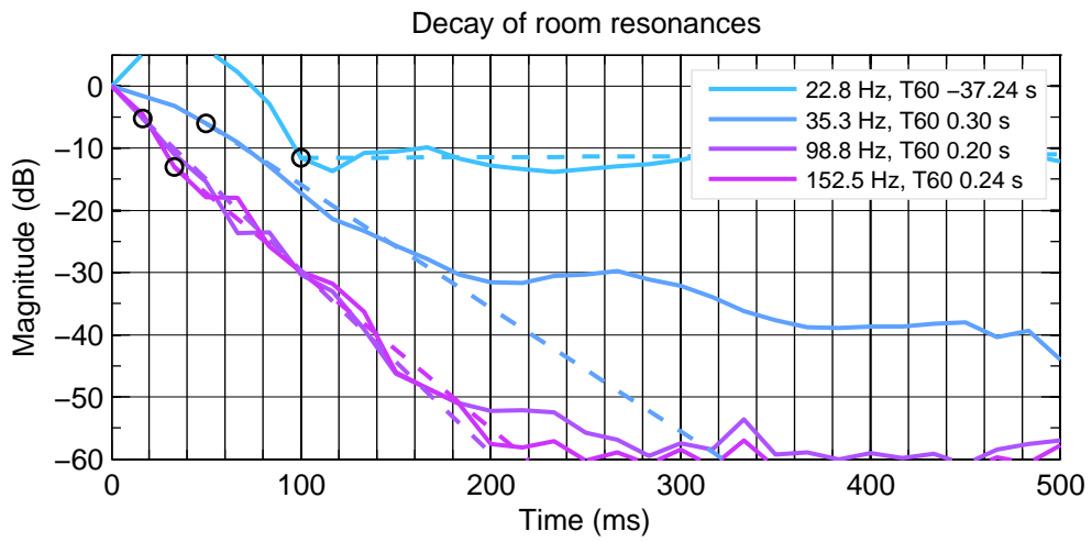
Figure 5.6: Right 8351B. Decay of detected resonances.
