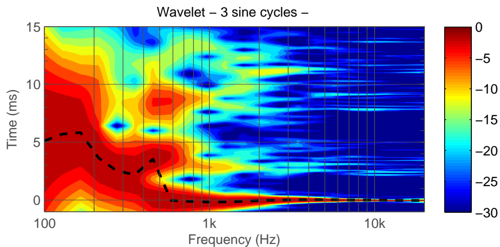
Figure 5.9: Right 8351B. Wavelet.
