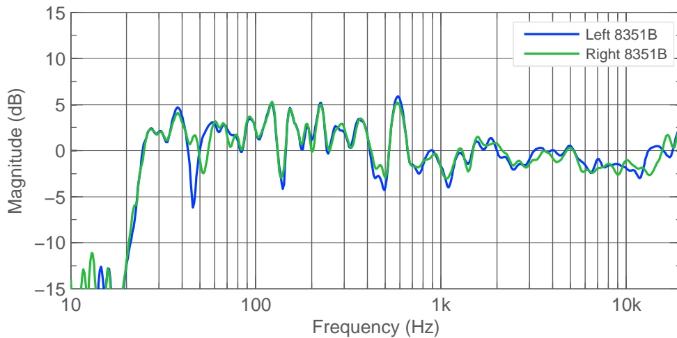
Figure 3.3: Frequency responses for monitors. AccuSmoothed.
