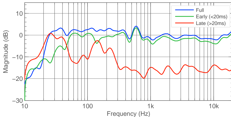
Figure 4.7: Left 8351B. Full, early and late frequency response.
