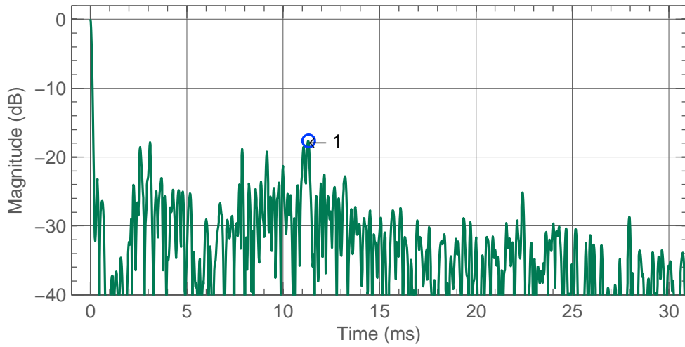
Figure 4.5: Right 8351B early reflections.
