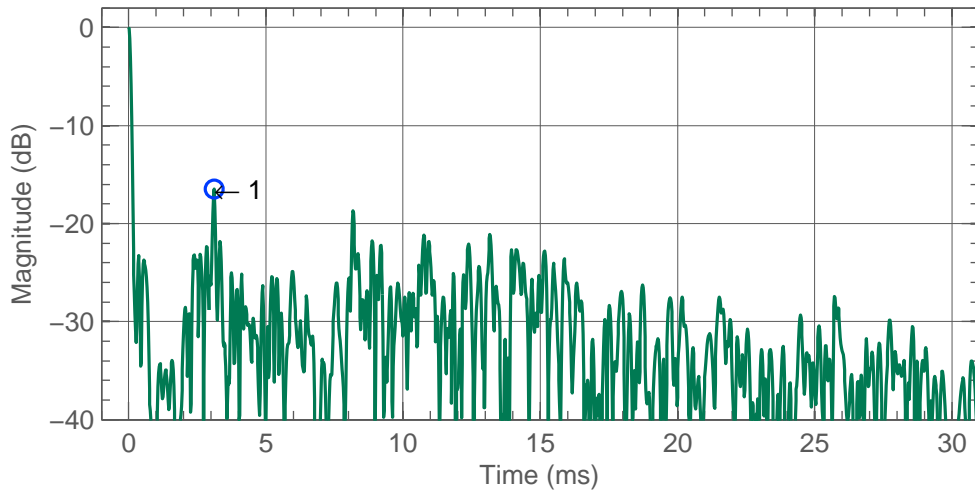
Figure 4.3: Left 8351B early reflections.
