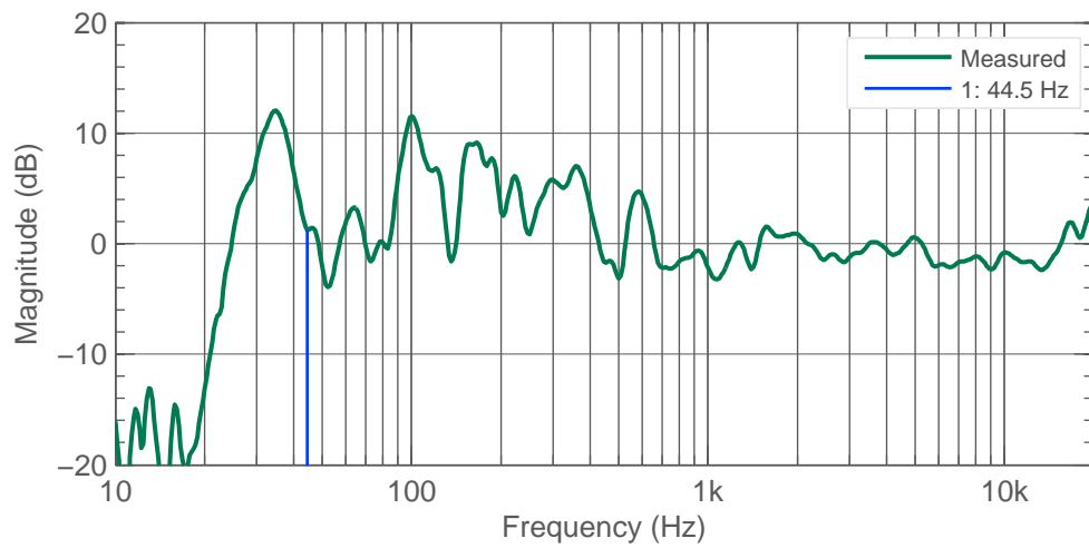
Figure 4.6: Right 8351B. Response and lowest cancellation frequency resulting from early reflection.
