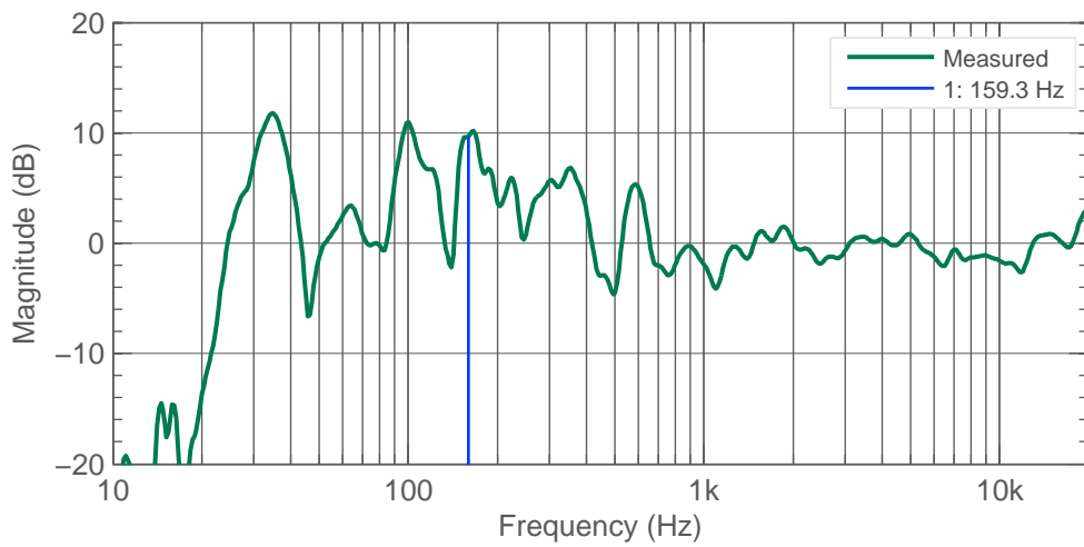
Figure 4.4: Left 8351B. Response and lowest cancellation frequency resulting from early reflection.
