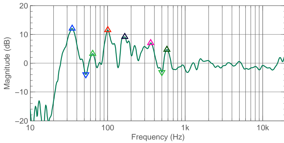
Figure 3.7: Right 8351B peaks and notches (before calibration).
