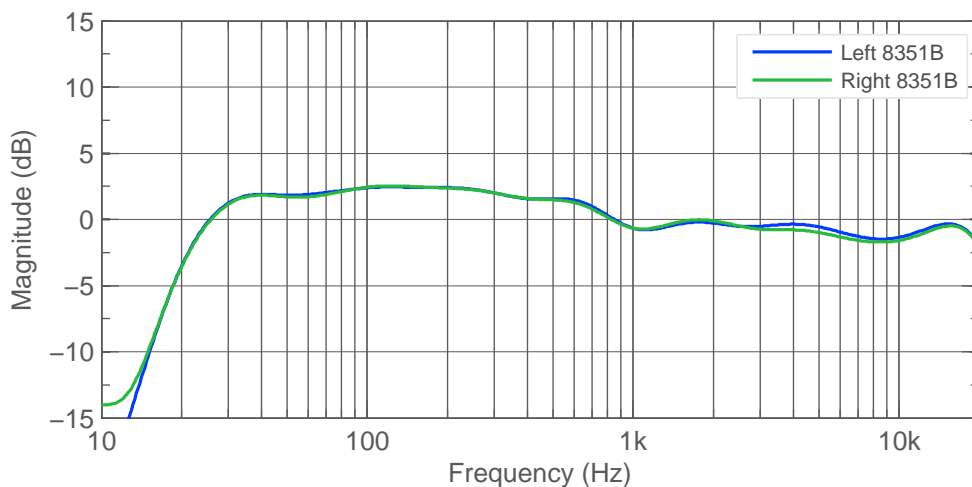
Figure 3.4: Frequency responses for monitors. One octave smoothing.
