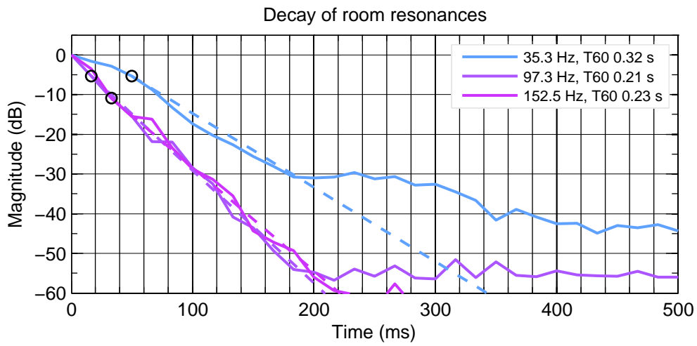
Figure 5.4: Left 8351B. Decay of detected resonances.
